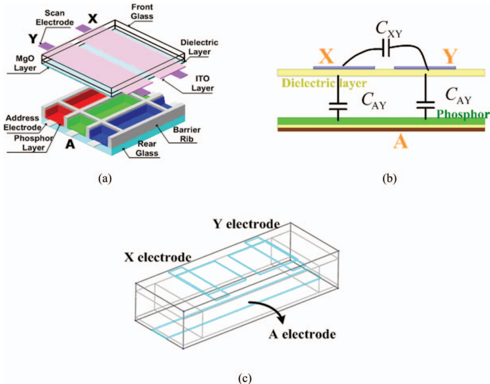
Figure 1. Schematic diagrams of (a) single pixel structure in 50 inch HD AC-PDP, (b) capacitances of between X-Y and A-Y electrodes in PDP cell, and (c) cell structure used in calculation of capacitance.
