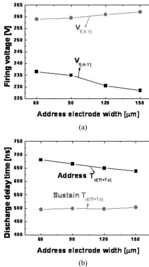
Figure 5. Comparison of (a) firing voltages between X-Y and A-Y electrodes and (b) address delay time during address and sustain discharge under various address electrode widths.
