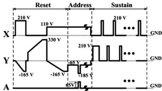
Figure 4. Schematic diagram of conventional driving waveform used in this paper.
