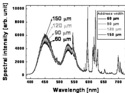
Figure 7. Comparison of spectral intensity of visible under various address electrode widths.
