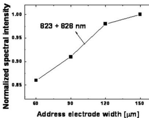
Figure 8. Comparison of (a) Xe (IR, 823 and 828 nm) and Ne (585 nm) spectral intensity and (b) Xe (IR, 823 adds to 828 nm) under various address electrode widths.
