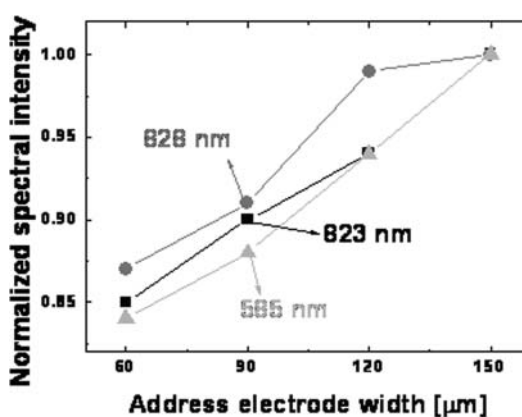
Figure 7. Comparison of spectral intensity of visible under various address electrode widths.
