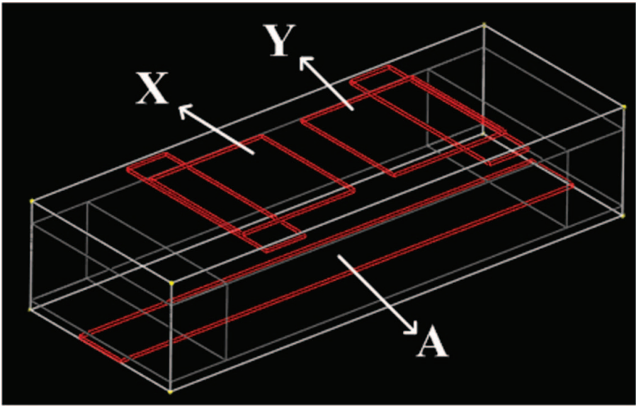
Figure 9. Schematic diagrams of cell structure for 3-D simulation.
