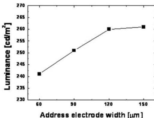
Figure 6. Comparison of luminance under full white background under various address electrode widths.
