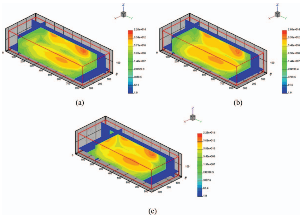
Figure 11. Comparison of Xe ion distribution based on simulated results during sustain period under various address electrode widths. (a) 90\ \mu\text{m} , (b) 130\ \mu\text{m} , and (c) 150\ \mu\text{m} .
