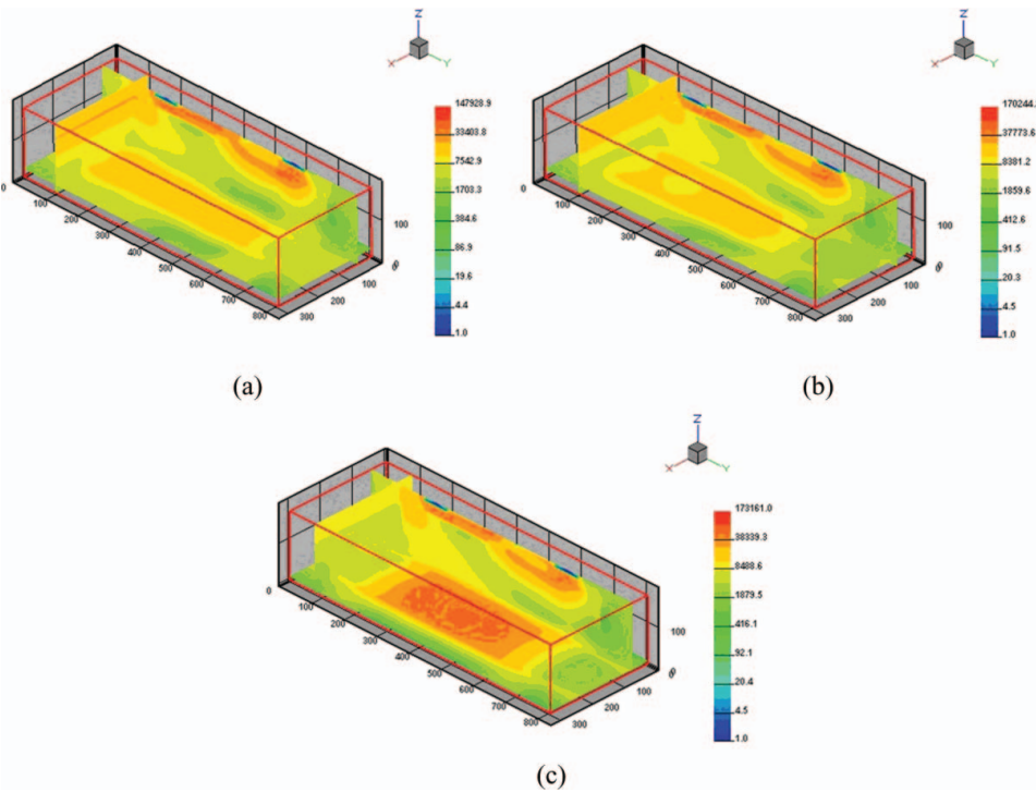
Figure 10. Comparison of electric field strength based on simulated results during sustain period under various address electrode widths. (a) 90 \mu\text{m} , (b) 130 \mu\text{m} , and (c) 150 \mu\text{m} .
