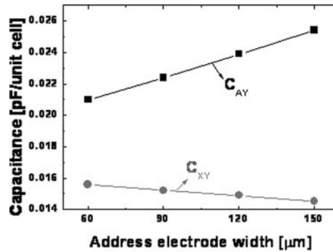
Figure 2. Comparison of capacitances between two sustain electrodes ( C_{XY} ) and between sustain and address electrodes ( C_{AY} ) per unit cell under various address electrode widths.
