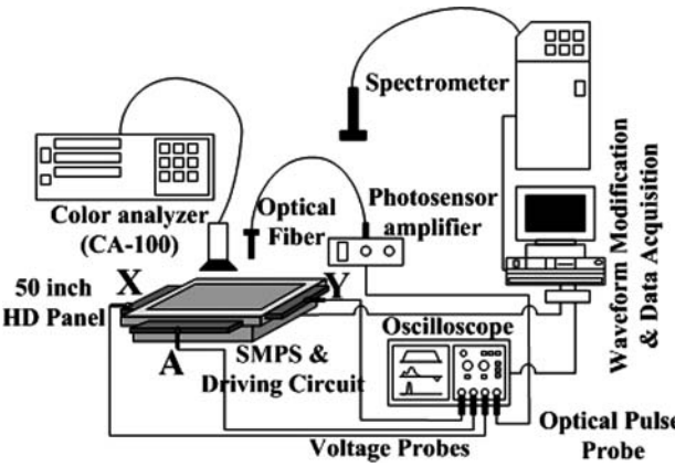
Figure 3. Schematic diagram of experimental setup employed in this paper.
